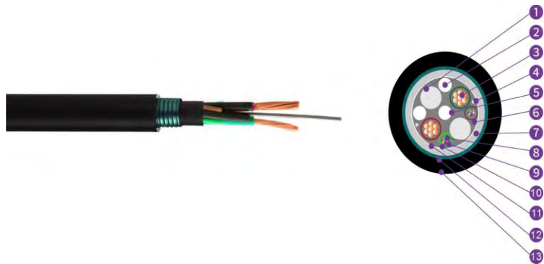
1, Filler 2, Filler 3, Copper Wire 4, Ripcord 5, Strength Member 6, Cable Filling Compound 7, PE Inner Sheath 8, Fibre 9, Tube Filling Compound 10, Loose Tube 11, APL 12, PSP 13, PE Outer Sheath
