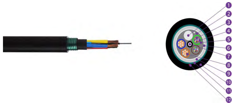
1, Filler 2, Cable Filling Compound 3, Fibre 4, Tube Filling Compound 5, Loose Tube 6, APL 7, Strength Member 8, Copper Wire 9, PE Inner Sheath 10, PE Outer Sheath 11, PSP 12, Ripcord
