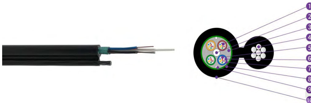
1, Copper Wire 2, Strength Member 3, Cable Filling Compound 4, Steel Wire 5, Fibre 6, Tube Filling Compound 7, Loose Tube 8, PSP 9, Ripcord 10, PE Sheath
